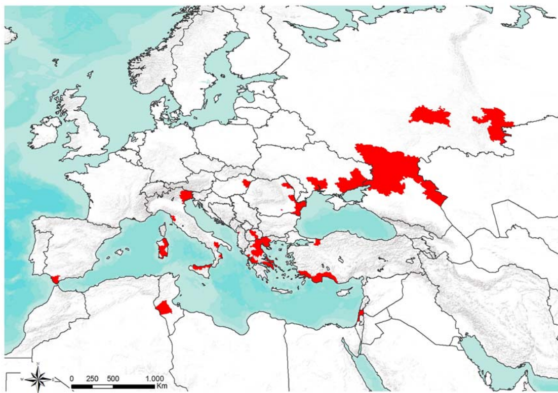
Figure 1 Geographic distribution of West Nile disease in the Mediterranean Basin
